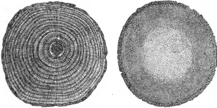
FIG. 83. — Typical exogenous and endogenous stems, in cross section, of Red Pine and a Palm; \times \frac{1}{4} . (Drawn from photographs.)
